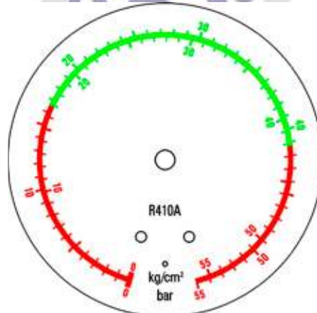
Abbildung 23: Manometers.
